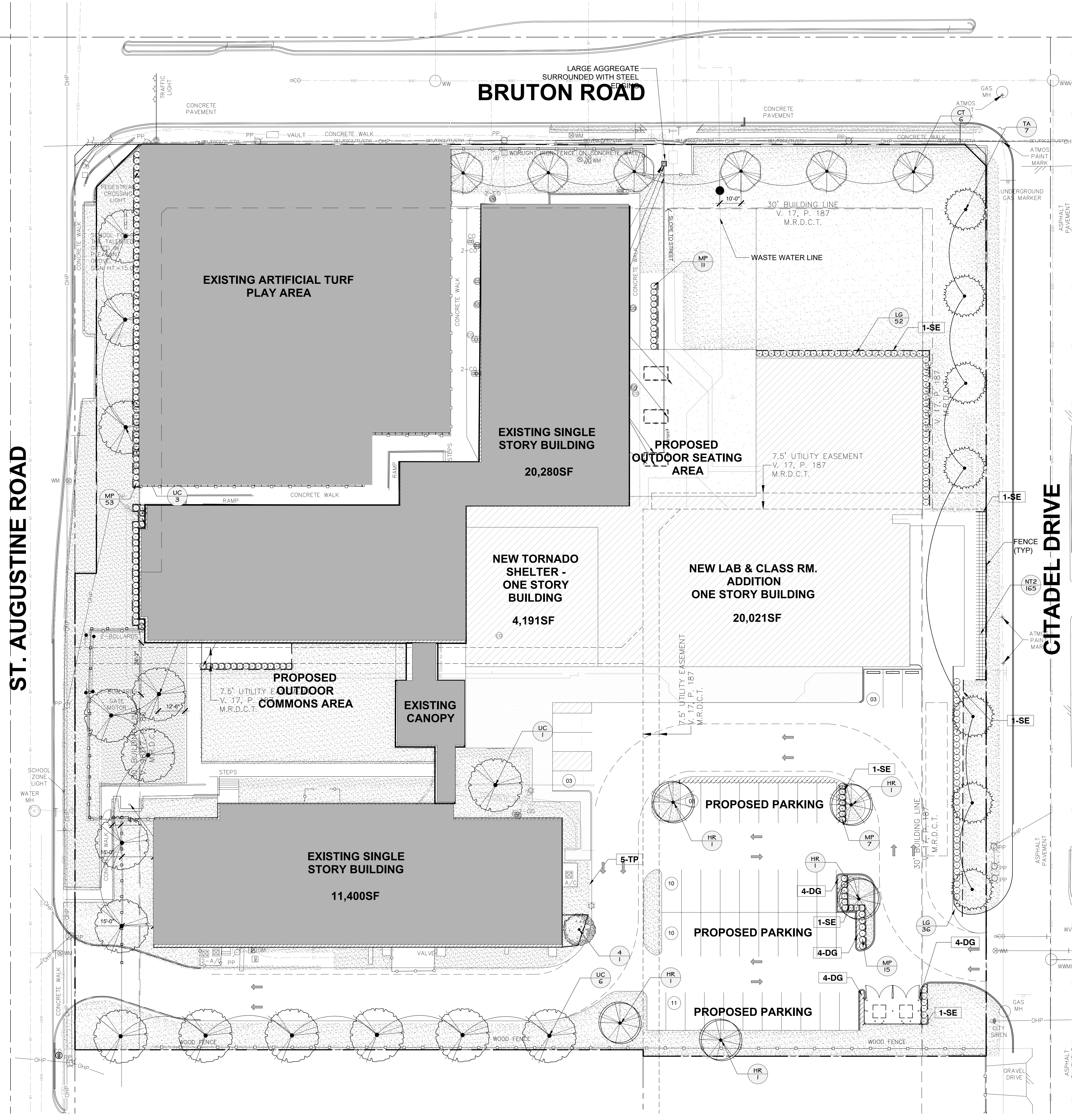
1 LANDSCAPE PLAN 1"=20'-0"
